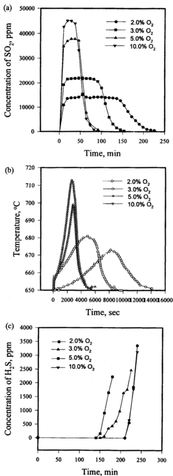
Fig. 2. (a) SO 2 breakthrough curve vs. concentration of oxygen (The effect of oxygen conc.). (b) Temperature profile during regeneration (The effect of oxygen conc.). (c) H 2 S breakthrough curves after regeneration (The effect of oxygen conc.).
