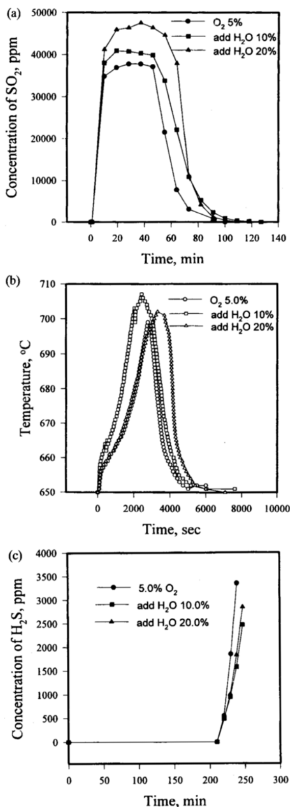
Fig. 4. (a) SO 2 breakthrough curve vs. concentration of steam (The effect of steam). (b) Temperature profile during regeneration (The effect of steam). (c) H 2 S breakthrough curves after regeneration (The effect of steam).
